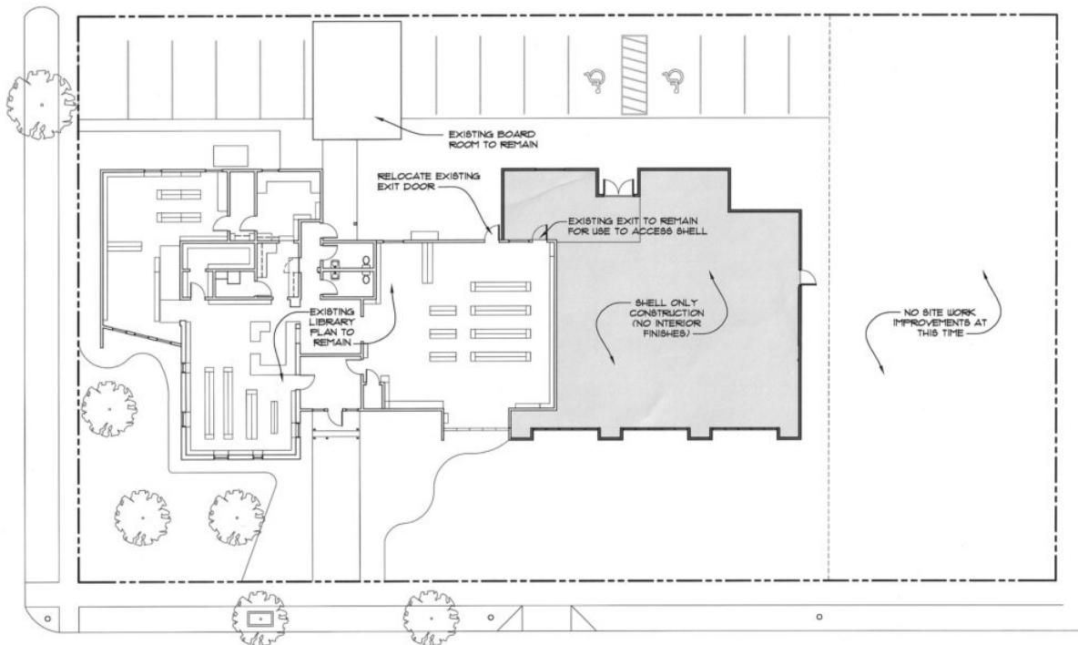
PHASE 1 - CLEARWATER MEMORIAL PUBLIC LIBRARY EXPANSION SCALE: 1/16" = 1'-0"
