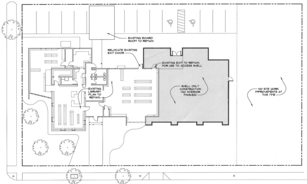
PHASE I - CLEARWATER MEMORIAL PUBLIC LIBRARY EXPANSION SCALE: 1/16" = 1'-0"
